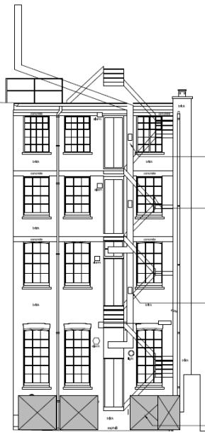
02 Proposed Elevation E1 Scale 1:100
