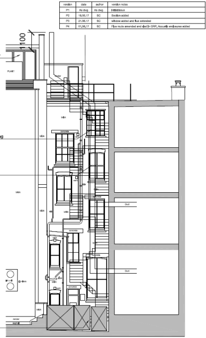
03 Proposed Section A Scale 1:100
